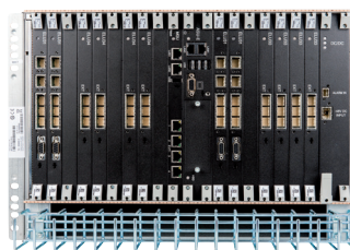
Chassis with embedded Media Gateway unit
